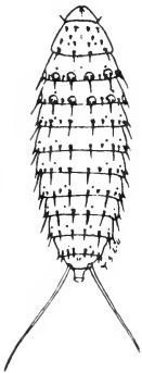
Fig. 551. Pterodontia flavipes Grag. 1st instar.
